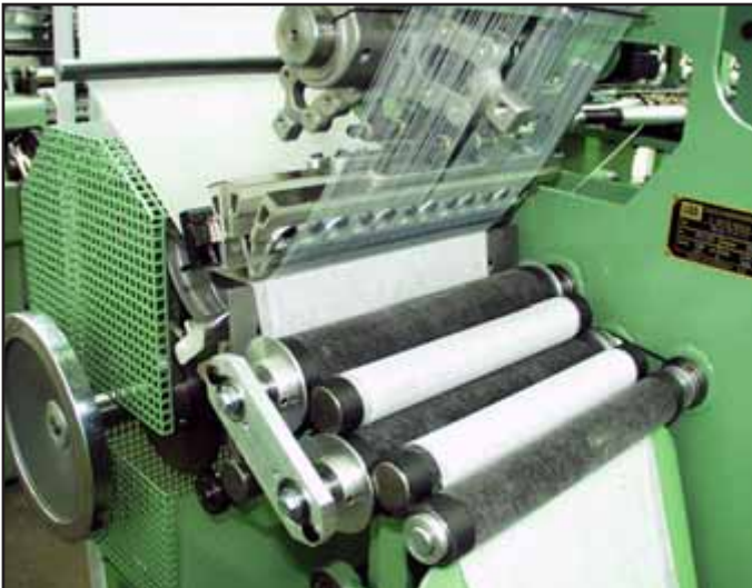
4-Walzen Warenabzug four roller fabric take-up system
